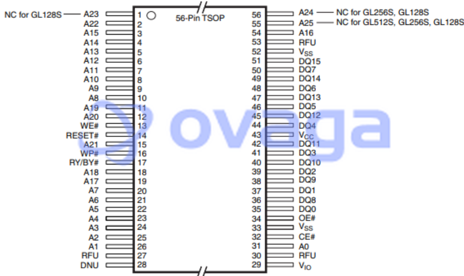
Figure 11.1 56-Pin Standard TSOP
